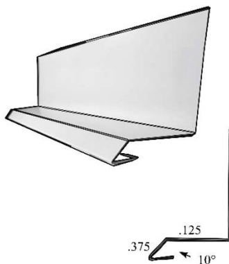
Deck Flashing
