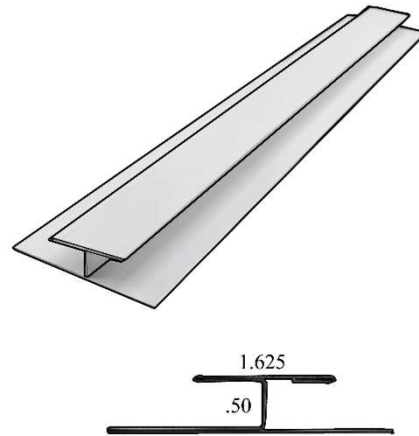
1/2" Stone Flashing
