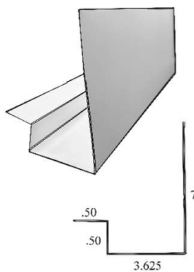
New Construction Window Trim
