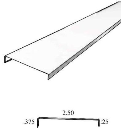
Replacement Window Trim
