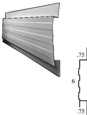
Deck Flashing
