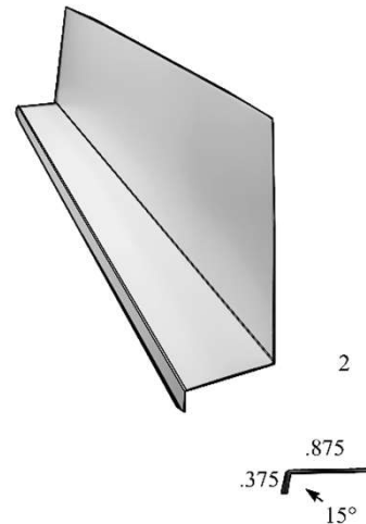
1/2" Stone Flashing
