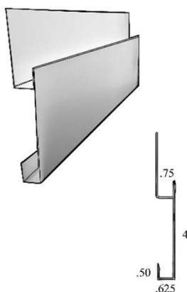
New Construction Window Trim
